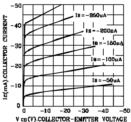
STATIC CHARACTERISTIC
